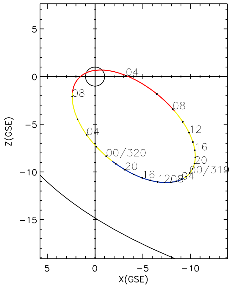
CLUSTER 2 orbit 2010 318 (11/14) 02:46 UT to 2010 320 (11/16) 09:01 UT
