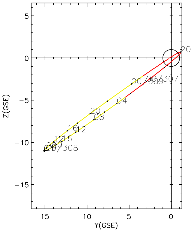
CLUSTER 2 orbit 2010 306 (11/02) 19:31 UT to 2010 309 (11/05) 01:46 UT
