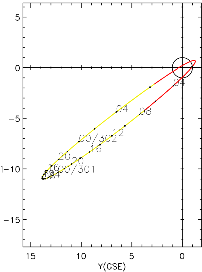
CLUSTER 2 orbit 2010 300 (10/27) 00:41 UT to 2010 302 (10/29) 06:56 UT
