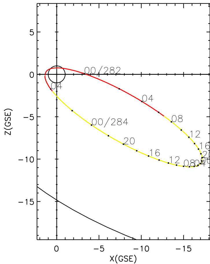
CLUSTER 2 orbit 2010 281 (10/08) 22:31 UT to 2010 284 (10/11) 04:46 UT
