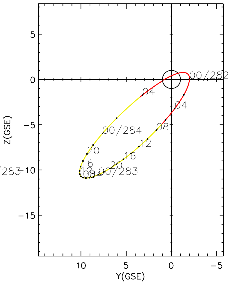
CLUSTER 2 orbit 2010 281 (10/08) 22:31 UT to 2010 284 (10/11) 04:46 UT
