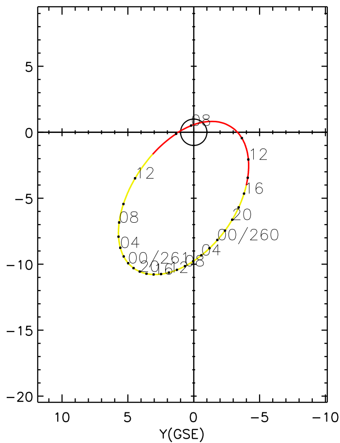
CLUSTER 2 orbit 2010 259 (09/16) 07:46 UT to 2010 261 (09/18) 14:01 UT
