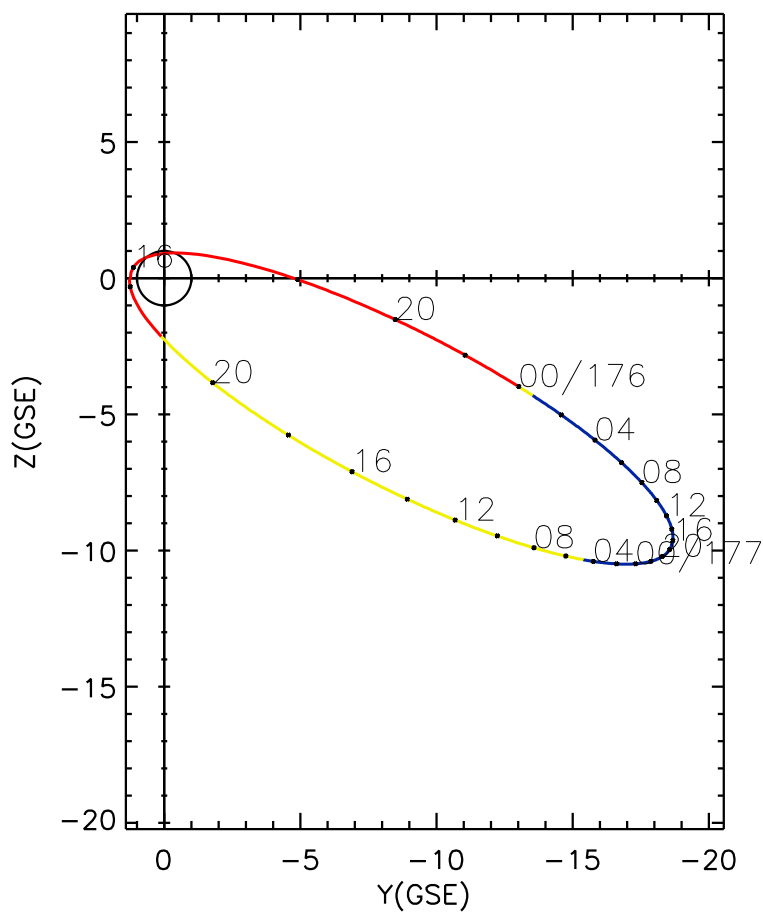
CLUSTER 2 orbit 2010 175 (06/24) 15:51 UT to 2010 177 (06/26) 22:06 UT
