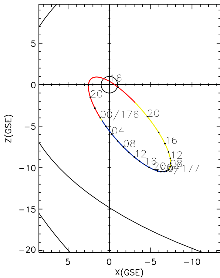
CLUSTER 2 orbit 2010 175 (06/24) 15:51 UT to 2010 177 (06/26) 22:06 UT
