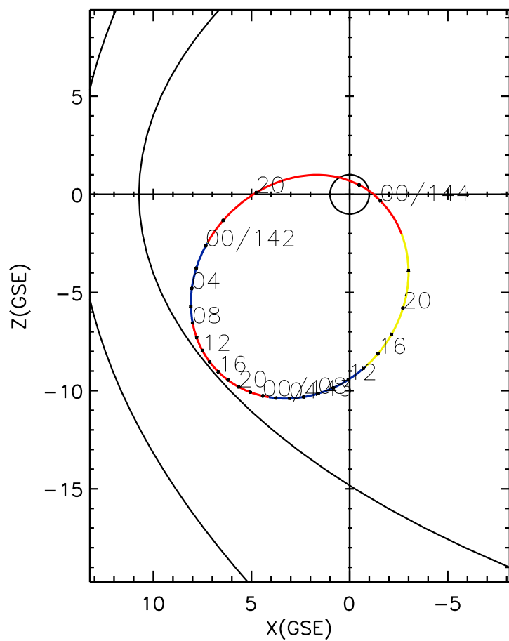
CLUSTER 2 orbit 2010 141 (05/21) 17:46 UT to 2010 144 (05/24) 00:06 UT
