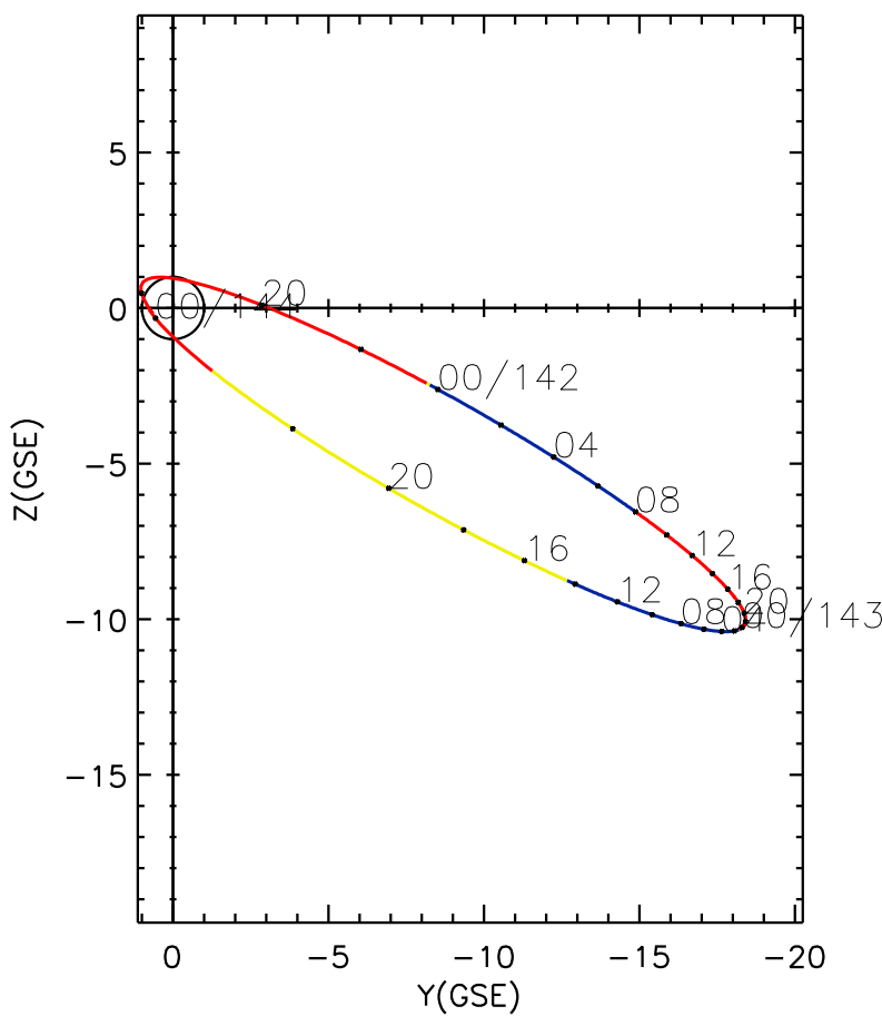
CLUSTER 2 orbit 2010 141 (05/21) 17:46 UT to 2010 144 (05/24) 00:06 UT
