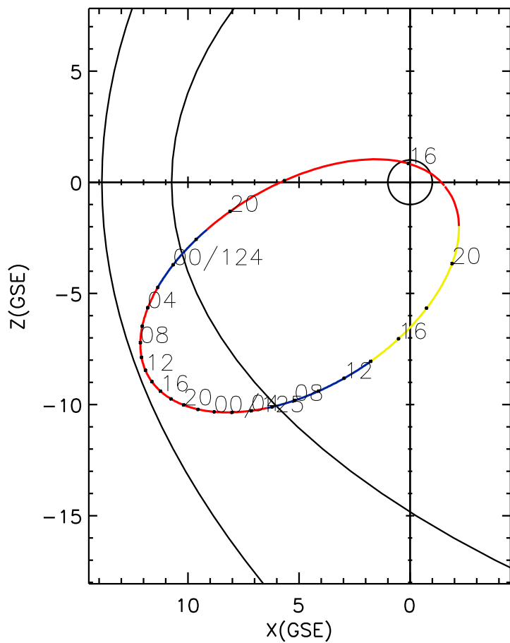
CLUSTER 2 orbit 2010 123 (05/03) 15:36 UT to 2010 125 (05/05) 21:51 UT
