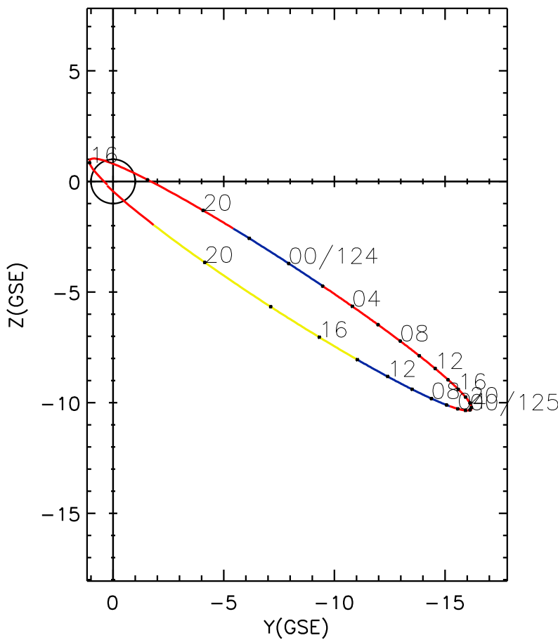
CLUSTER 2 orbit 2010 123 (05/03) 15:36 UT to 2010 125 (05/05) 21:51 UT
