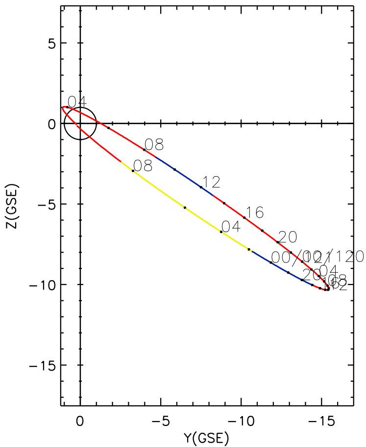
CLUSTER 2 orbit 2010 119 (04/29) 03:06 UT to 2010 121 (05/01) 09:21 UT
