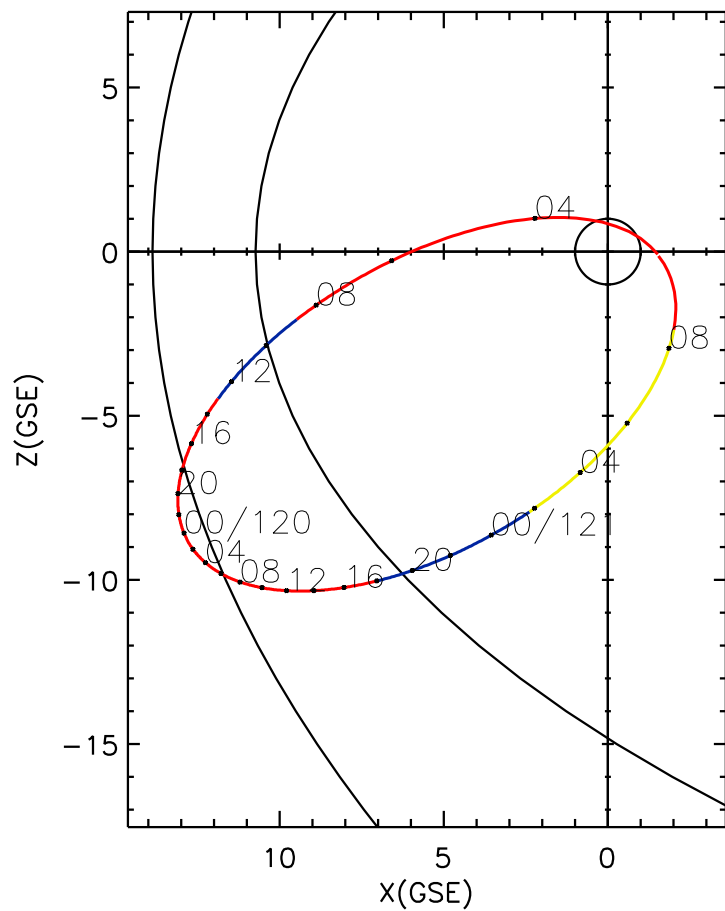
CLUSTER 2 orbit 2010 119 (04/29) 03:06 UT to 2010 121 (05/01) 09:21 UT
