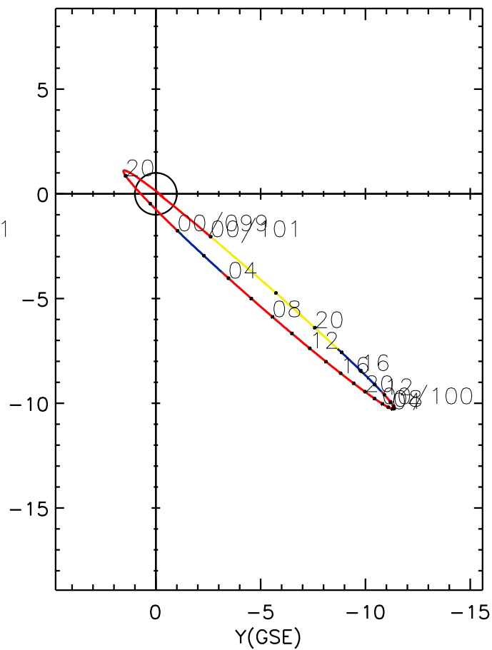
CLUSTER 2 orbit 2010 098 (04/08) 18:31 UT to 2010 101 (04/11) 00:51 UT
