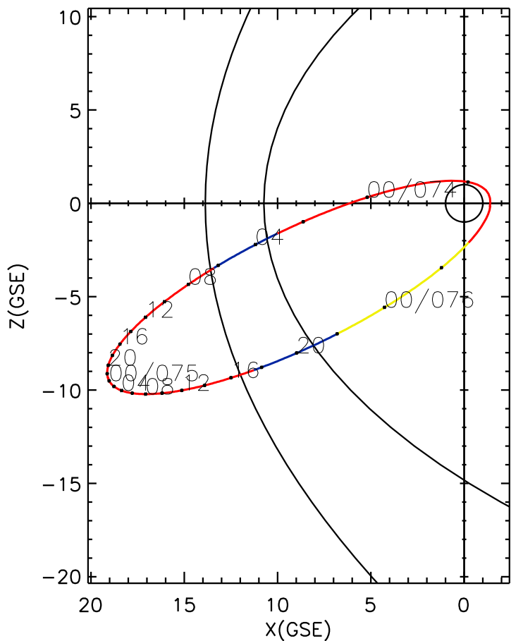
CLUSTER 2 orbit 2010 073 (03/14) 21:21 UT to 2010 076 (03/17) 03:41 UT
