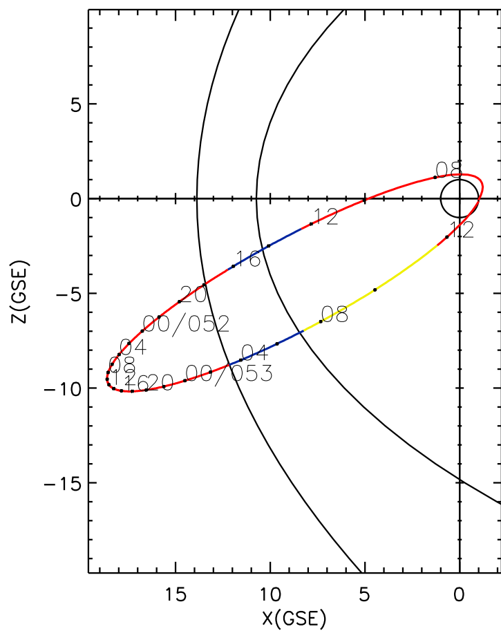
CLUSTER 2 orbit 2010 051 (02/20) 06:31 UT to 2010 053 (02/22) 12:46 UT
