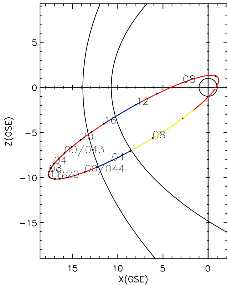
CLUSTER 2 orbit 2010 042 (02/11) 05:21 UT to 2010 044 (02/13) 11:36 UT
