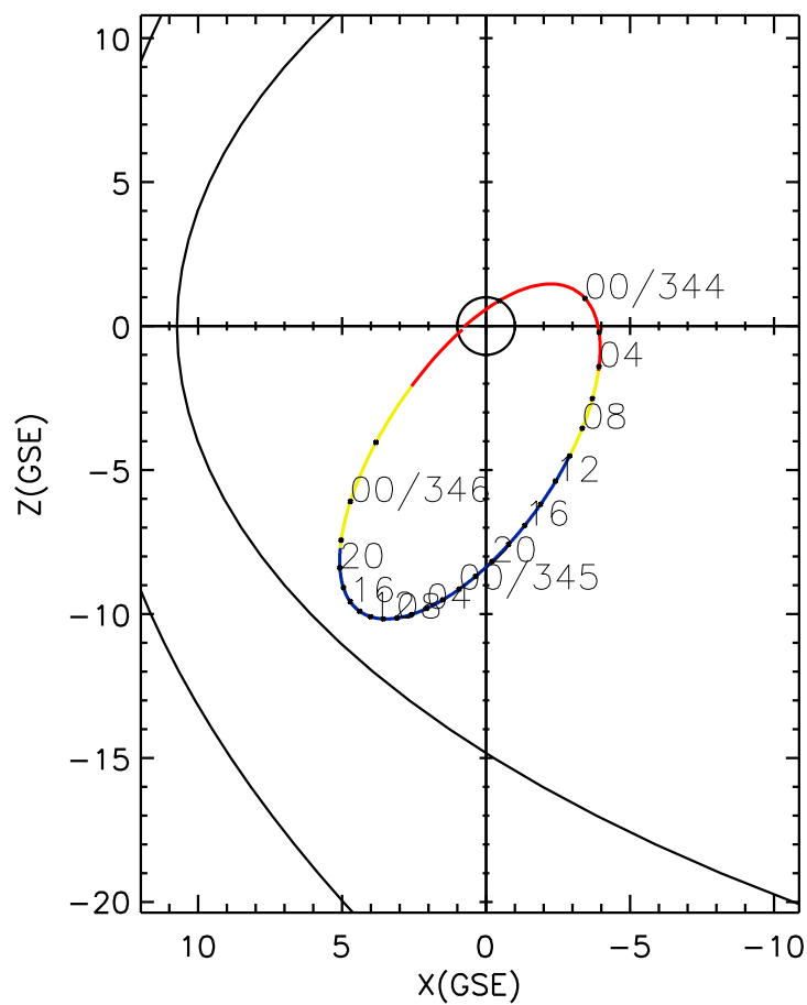
CLUSTER 2 orbit 2009 343 (12/09) 21:41 UT to 2009 346 (12/12) 03:56 UT
