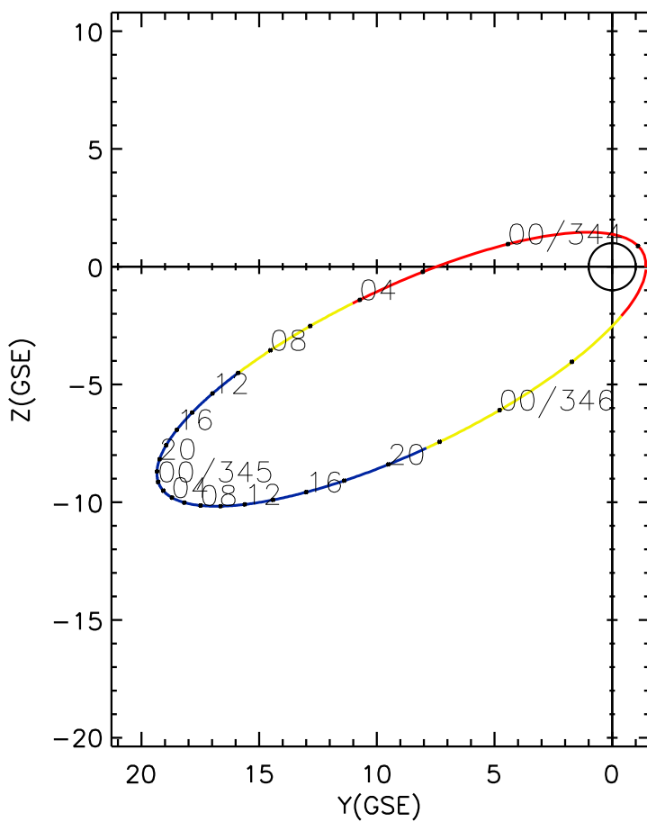
CLUSTER 2 orbit 2009 343 (12/09) 21:41 UT to 2009 346 (12/12) 03:56 UT
