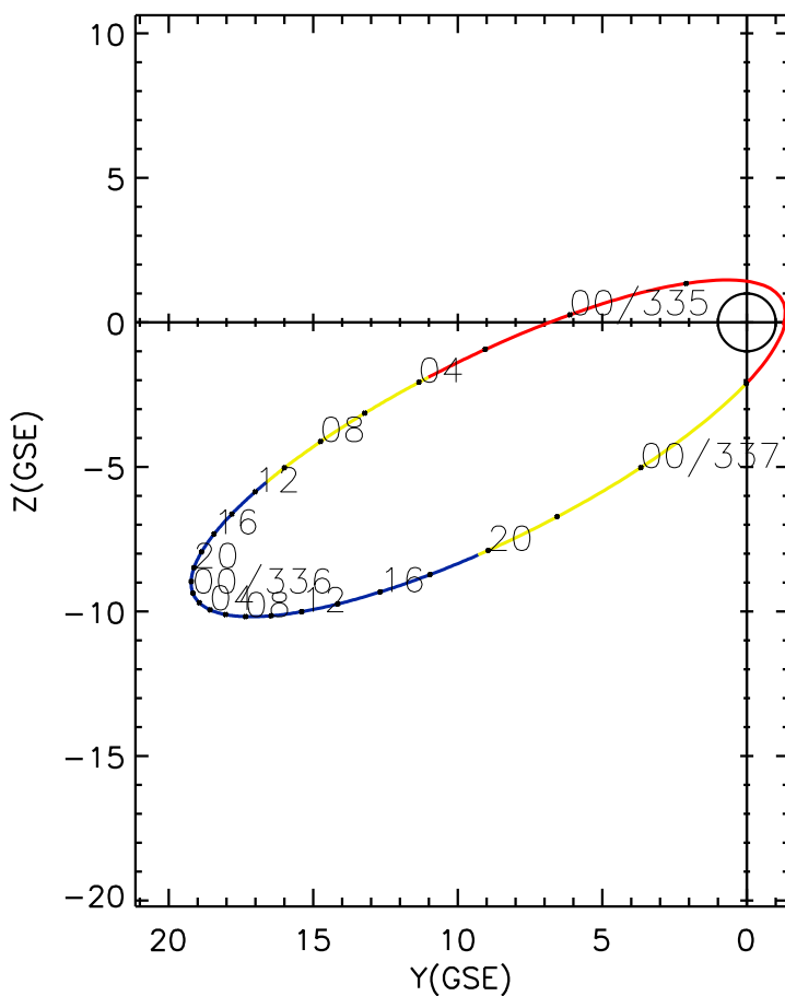
CLUSTER 2 orbit 2009 334 (11/30) 20:26 UT to 2009 337 (12/03) 02:46 UT
