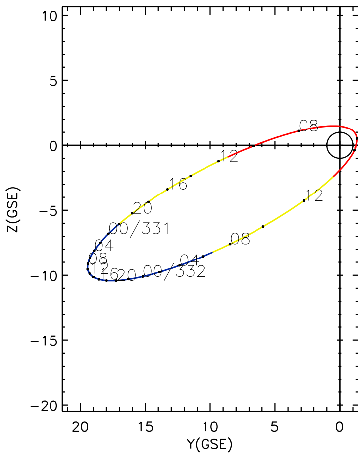
CLUSTER 2 orbit 2009 330 (11/26) 05:46 UT to 2009 332 (11/28) 14:06 UT
