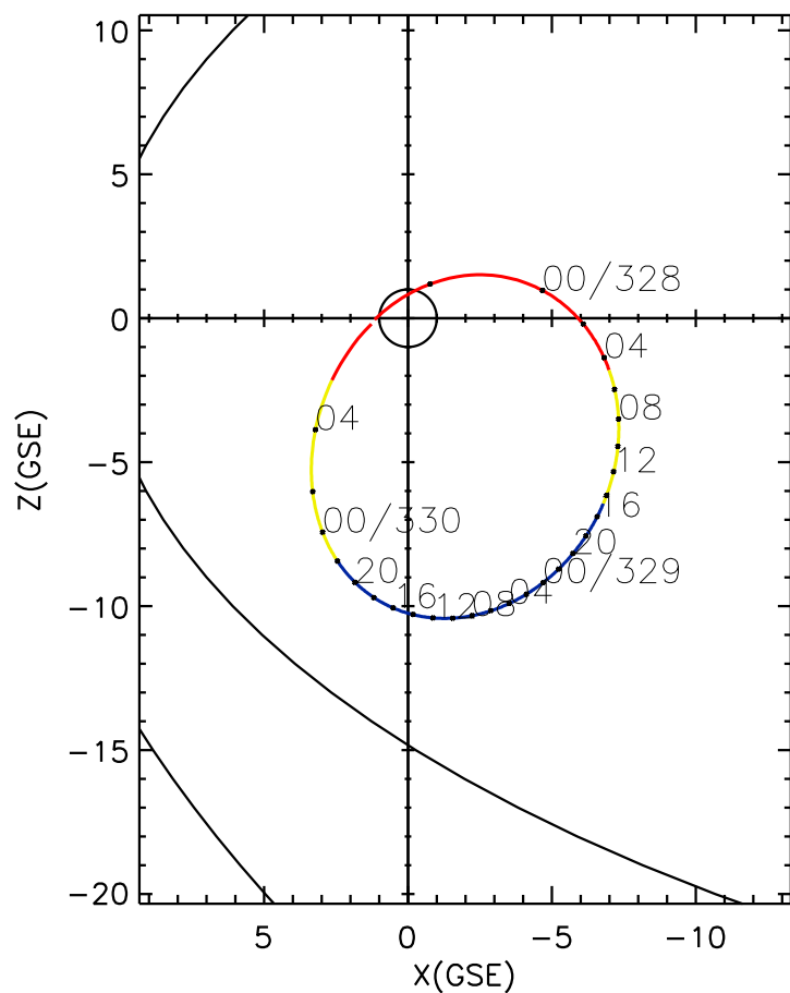
CLUSTER 2 orbit 2009 327 (11/23) 21:31 UT to 2009 330 (11/26) 05:46 UT
