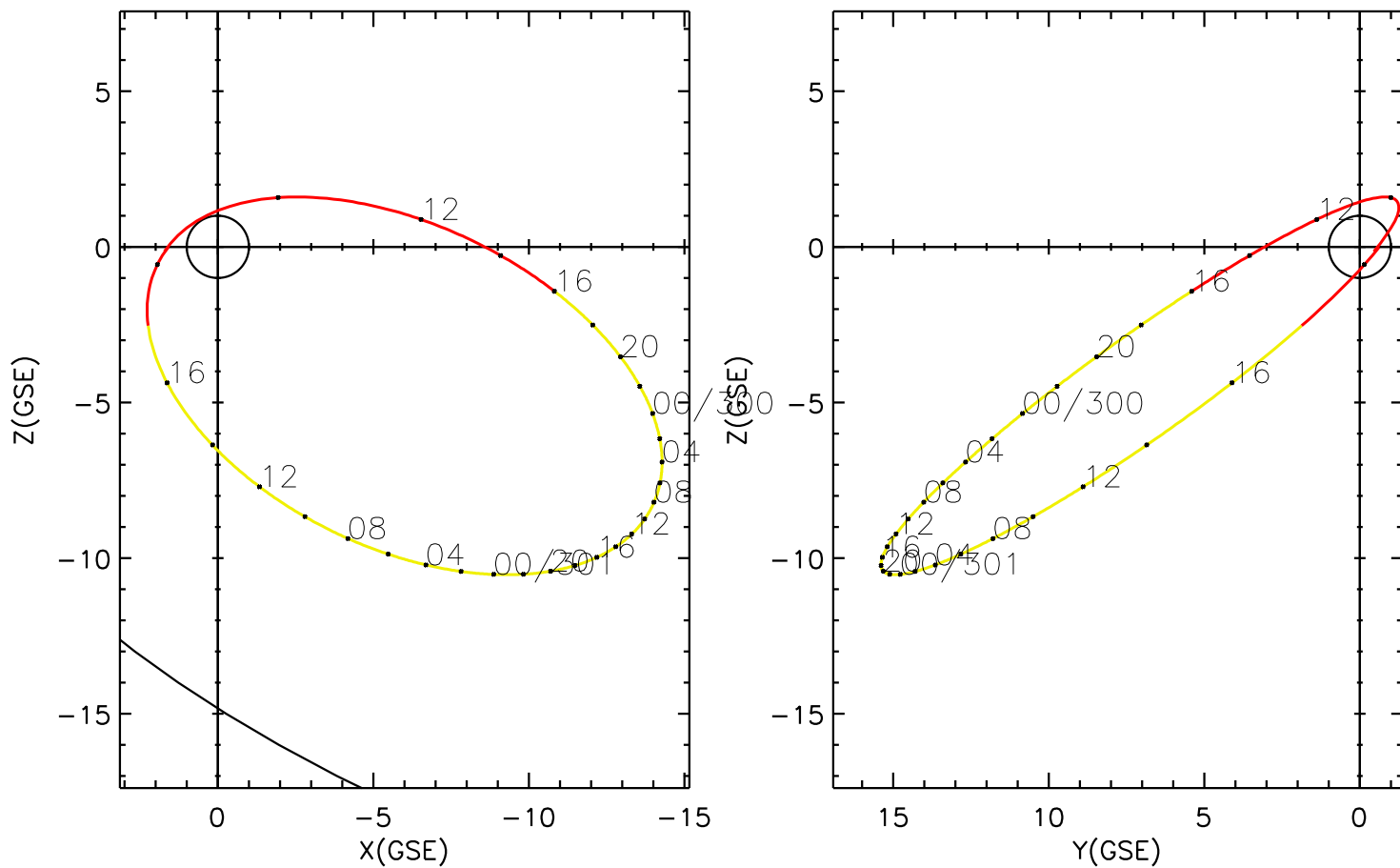
CLUSTER 2 orbit 2009 299 (10/26) 09:01 UT to 2009 301 (10/28) 18:11 UT
