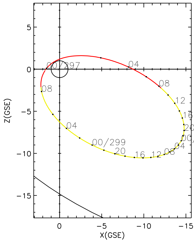
CLUSTER 2 orbit 2009 296 (10/23) 23:56 UT to 2009 299 (10/26) 09:01 UT
