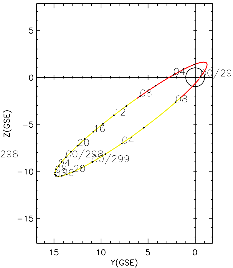
CLUSTER 2 orbit 2009 296 (10/23) 23:56 UT to 2009 299 (10/26) 09:01 UT
