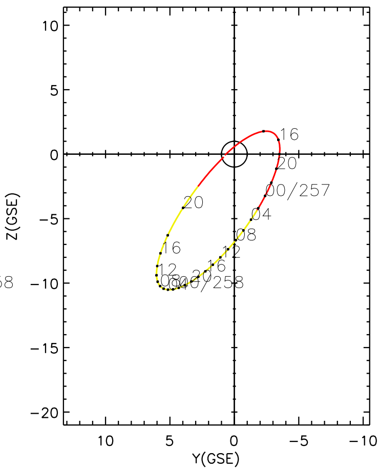
CLUSTER 2 orbit 2009 256 (09/13) 12:51 UT to 2009 258 (09/15) 21:56 UT
