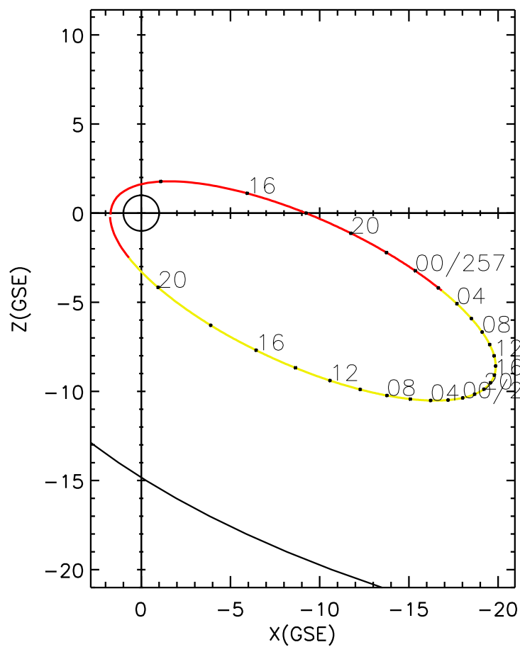
CLUSTER 2 orbit 2009 256 (09/13) 12:51 UT to 2009 258 (09/15) 21:56 UT
