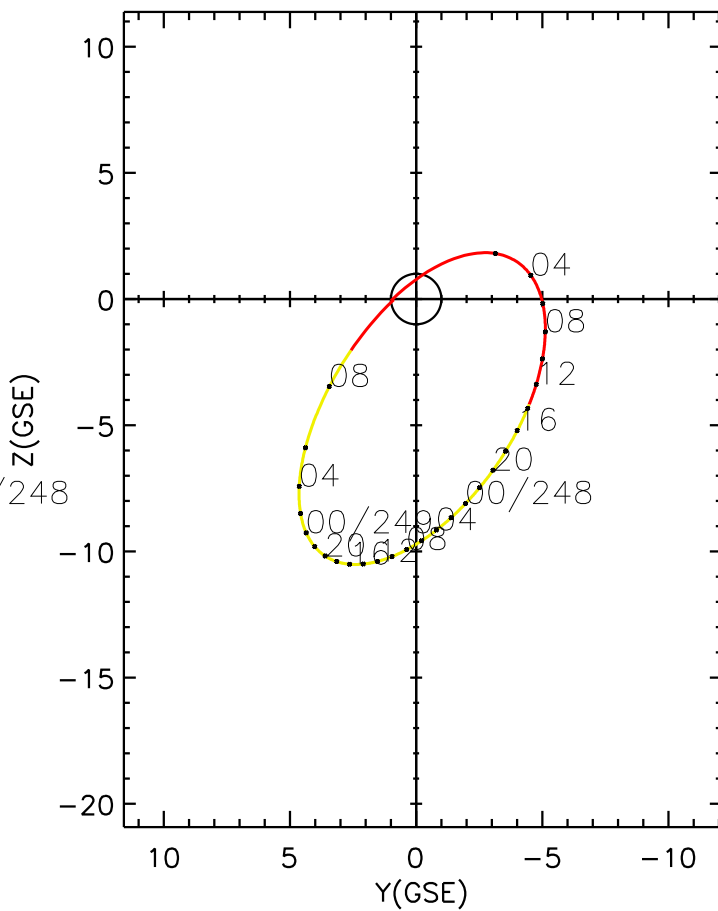
CLUSTER 2 orbit 2009 247 (09/04) 00:21 UT to 2009 249 (09/06) 09:31 UT
