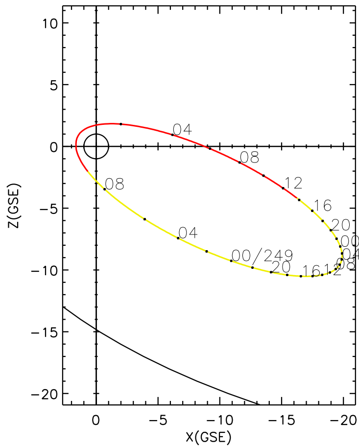
CLUSTER 2 orbit 2009 247 (09/04) 00:21 UT to 2009 249 (09/06) 09:31 UT
