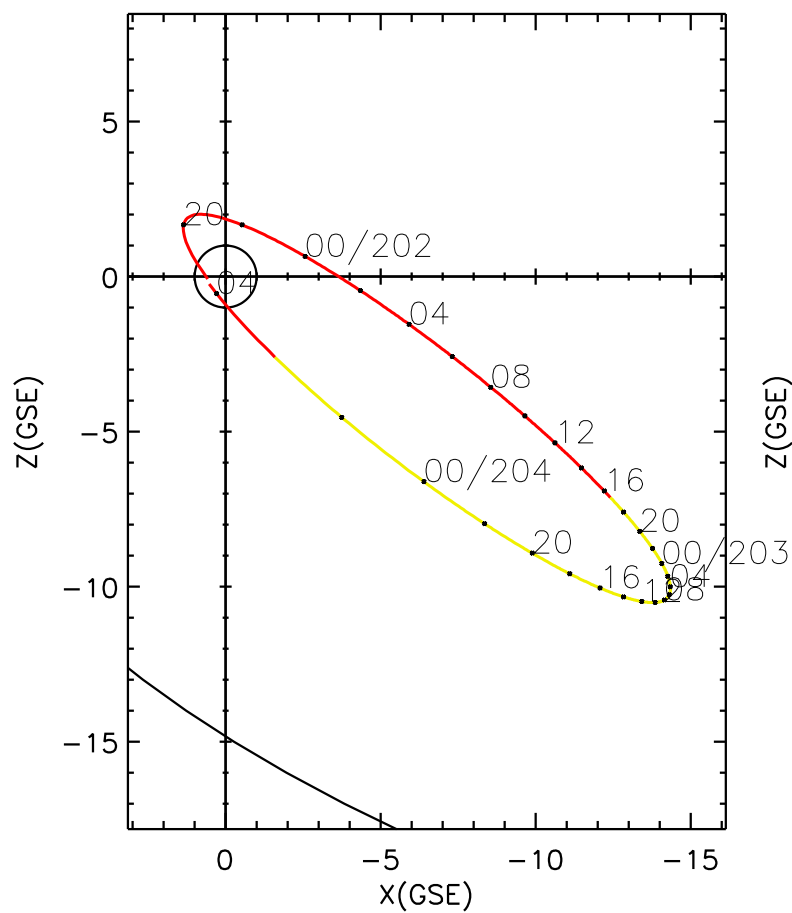
CLUSTER 2 orbit 2009 201 (07/20) 19:16 UT to 2009 204 (07/23) 04:06 UT
