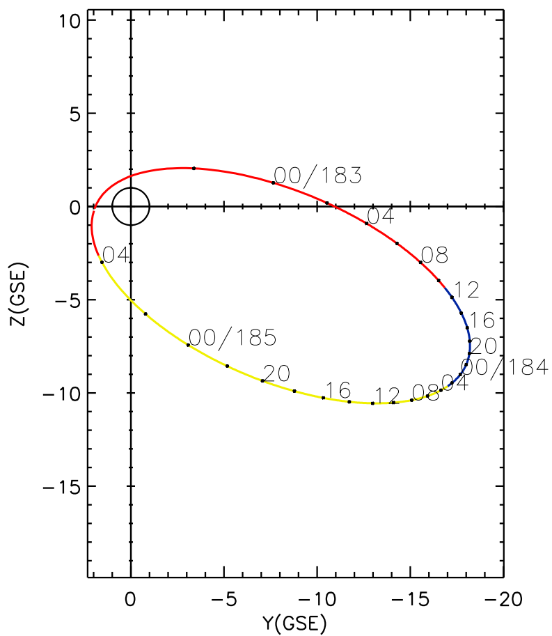
CLUSTER 2 orbit 2009 182 (07/01) 20:16 UT to 2009 185 (07/04) 05:06 UT
