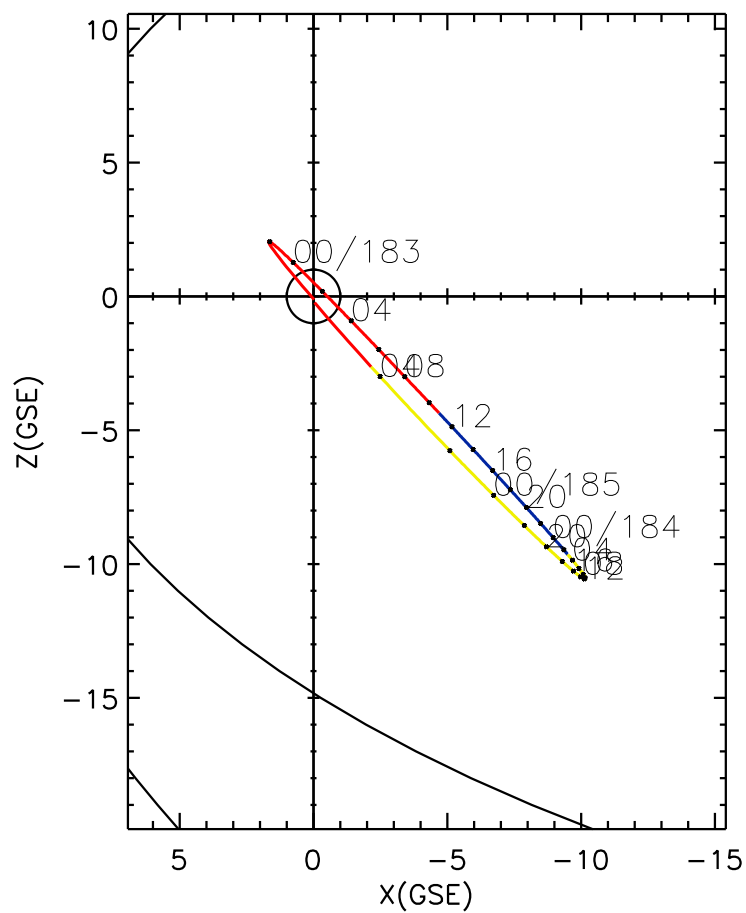
CLUSTER 2 orbit 2009 182 (07/01) 20:16 UT to 2009 185 (07/04) 05:06 UT
