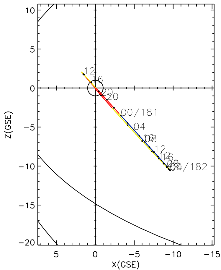
CLUSTER 2 orbit 2009 180 (06/29) 11:11 UT to 2009 182 (07/01) 20:16 UT
