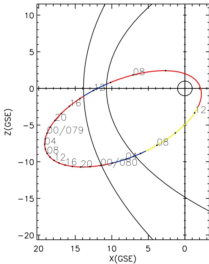
CLUSTER 2 orbit 2009 078 (03/19) 04:11 UT to 2009 080 (03/21) 13:21 UT
