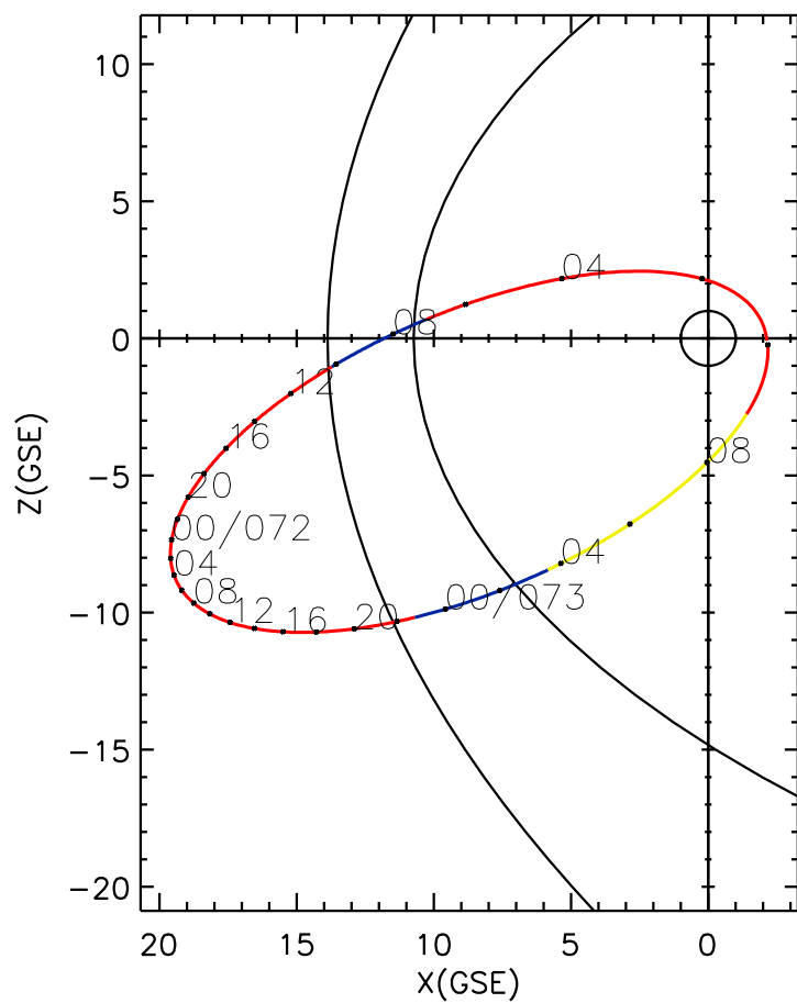
CLUSTER 2 orbit 2009 071 (03/12) 00:56 UT to 2009 073 (03/14) 10:01 UT
