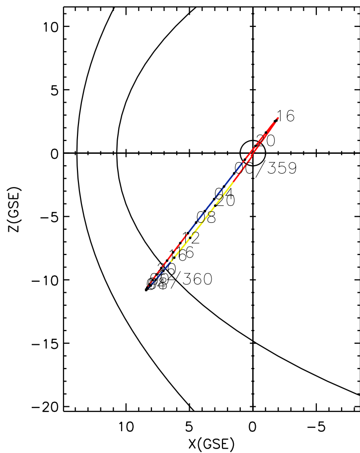
CLUSTER 2 orbit 2008 358 (12/23) 12:36 UT to 2008 360 (12/25) 21:41 UT
