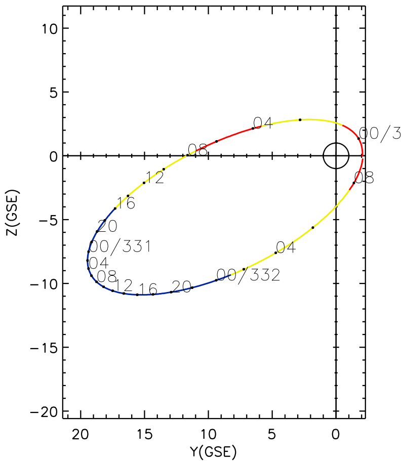
CLUSTER 2 orbit 2008 329 (11/24) 23:31 UT to 2008 332 (11/27) 08:41 UT
