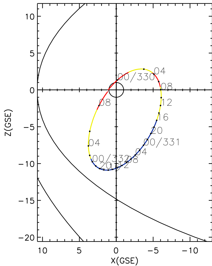
CLUSTER 2 orbit 2008 329 (11/24) 23:31 UT to 2008 332 (11/27) 08:41 UT
