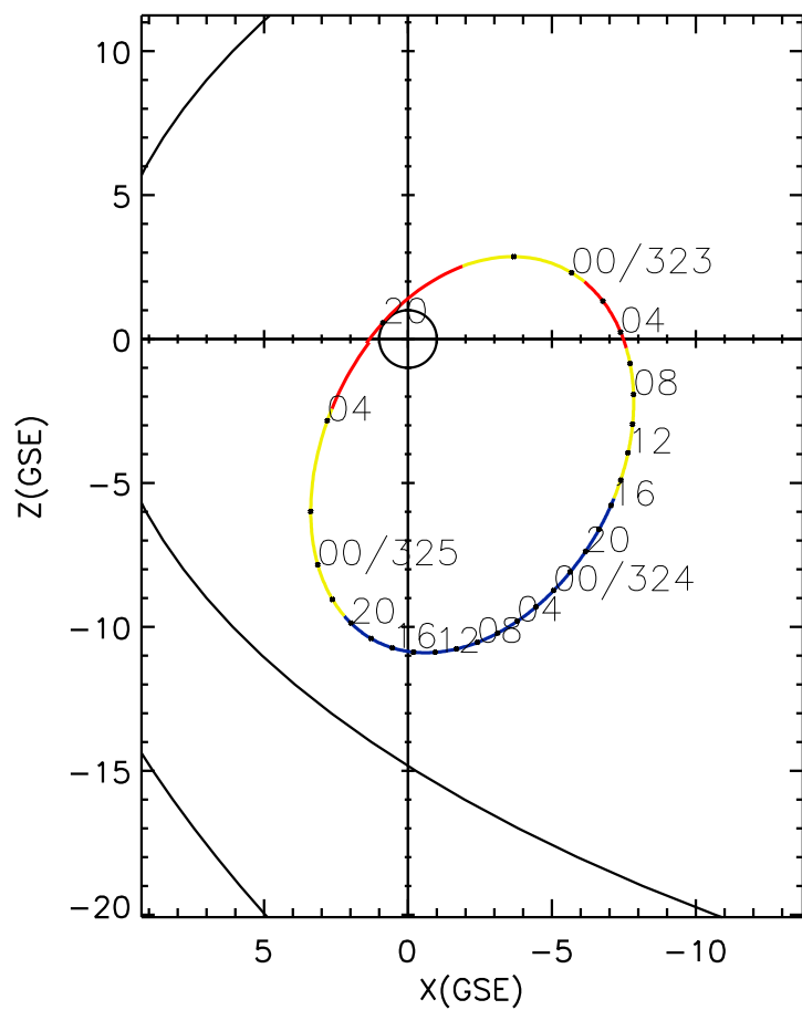
CLUSTER 2 orbit 2008 322 (11/17) 19:46 UT to 2008 325 (11/20) 05:01 UT
