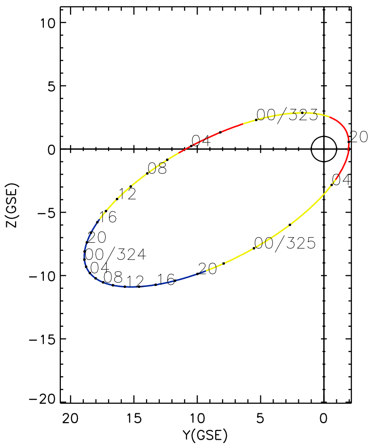
CLUSTER 2 orbit 2008 322 (11/17) 19:46 UT to 2008 325 (11/20) 05:01 UT
