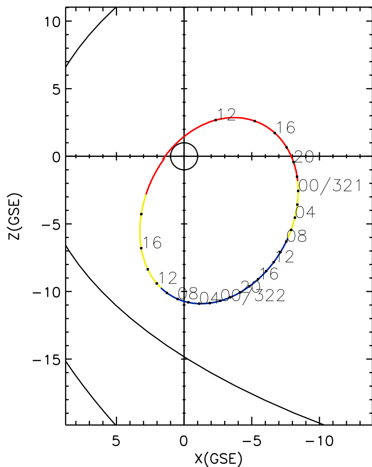
CLUSTER 2 orbit 2008 320 (11/15) 10:31 UT to 2008 322 (11/17) 19:46 UT
