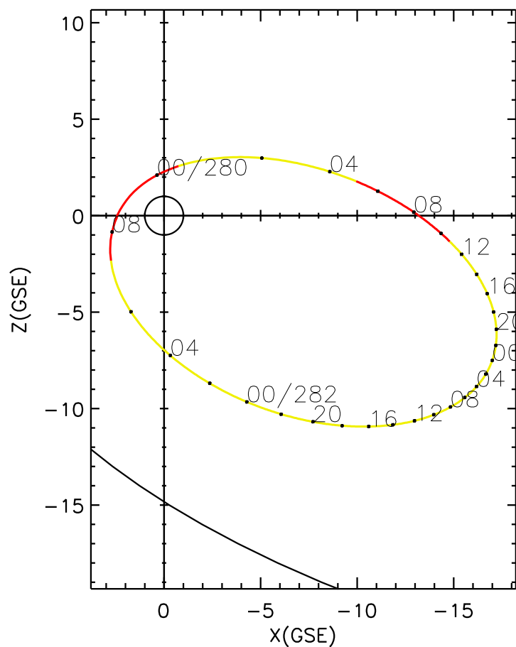
CLUSTER 2 orbit 2008 279 (10/05) 23:06 UT to 2008 282 (10/08) 08:16 UT
