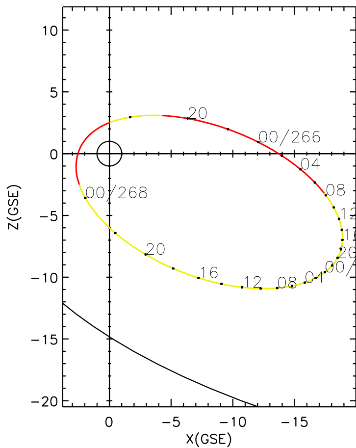
CLUSTER 2 orbit 2008 265 (09/21) 16:16 UT to 2008 268 (09/24) 01:26 UT
