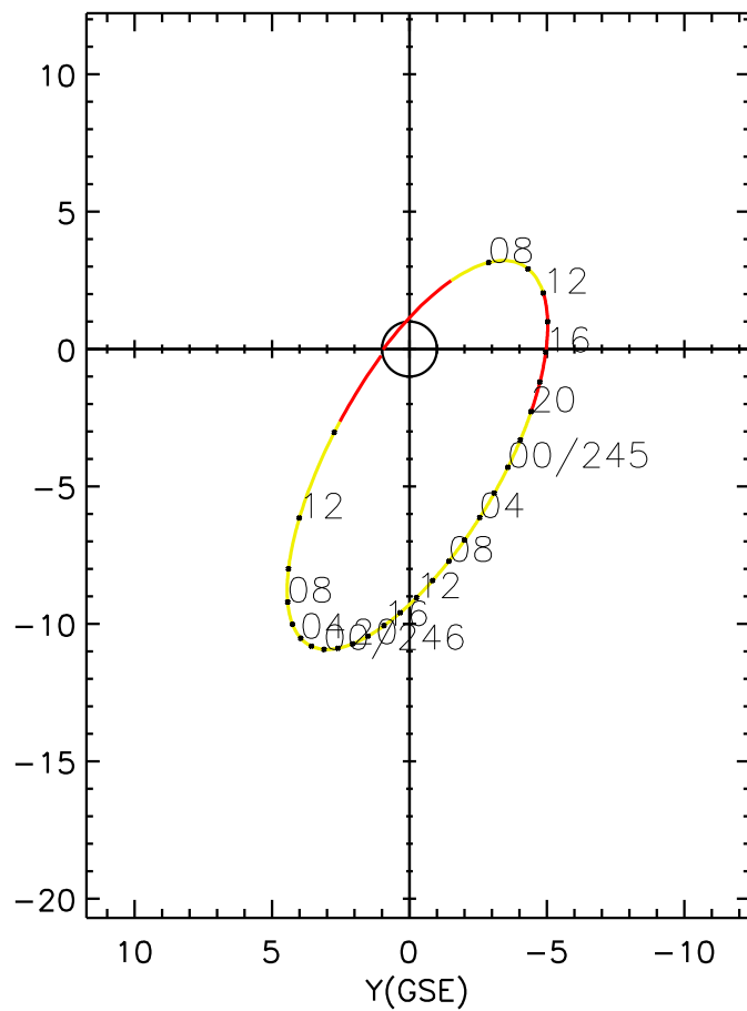
CLUSTER 2 orbit 2008 244 (08/31) 06:01 UT to 2008 246 (09/02) 15:06 UT
