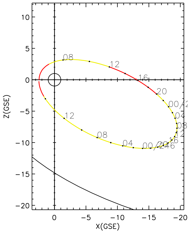
CLUSTER 2 orbit 2008 244 (08/31) 06:01 UT to 2008 246 (09/02) 15:06 UT
