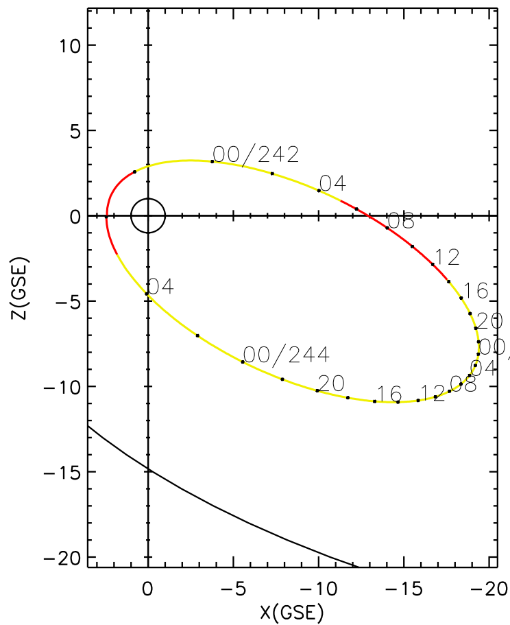
CLUSTER 2 orbit 2008 241 (08/28) 20:51 UT to 2008 244 (08/31) 06:01 UT
