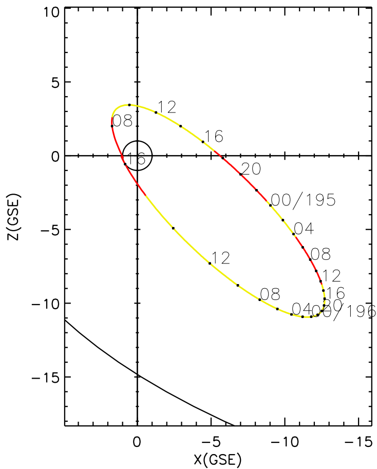
CLUSTER 2 orbit 2008 194 (07/12) 07:11 UT to 2008 196 (07/14) 16:11 UT
