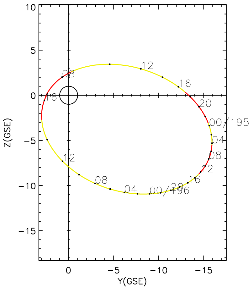
CLUSTER 2 orbit 2008 194 (07/12) 07:11 UT to 2008 196 (07/14) 16:11 UT
