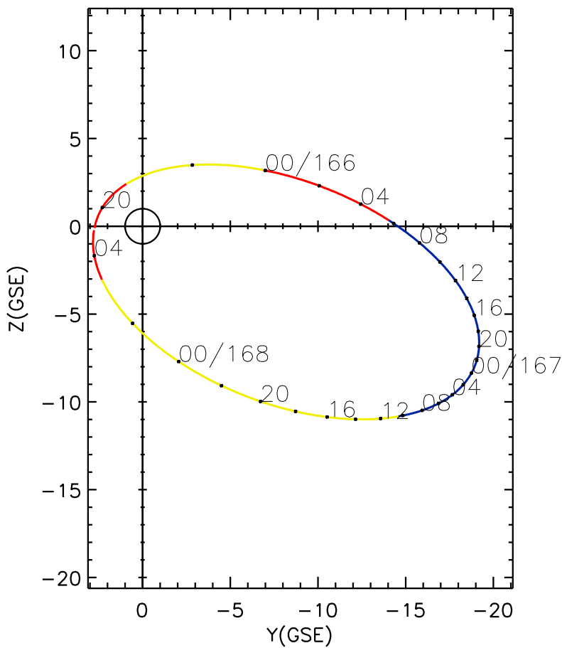
CLUSTER 2 orbit 2008 165 (06/13) 19:36 UT to 2008 168 (06/16) 04:31 UT
