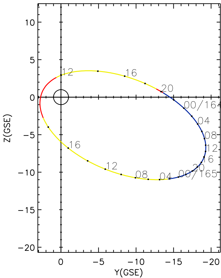
CLUSTER 2 orbit 2008 163 (06/11) 10:36 UT to 2008 165 (06/13) 19:36 UT
