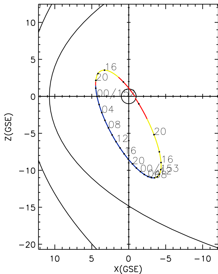
CLUSTER 2 orbit 2008 151 (05/30) 13:16 UT to 2008 153 (06/01) 22:16 UT
