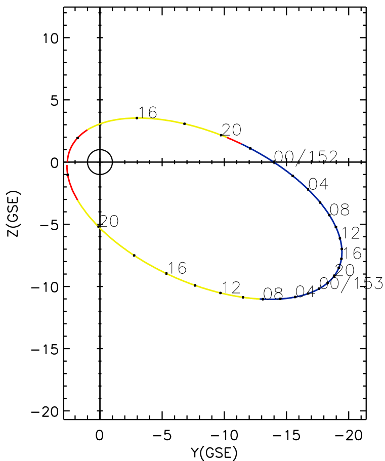
CLUSTER 2 orbit 2008 151 (05/30) 13:16 UT to 2008 153 (06/01) 22:16 UT
