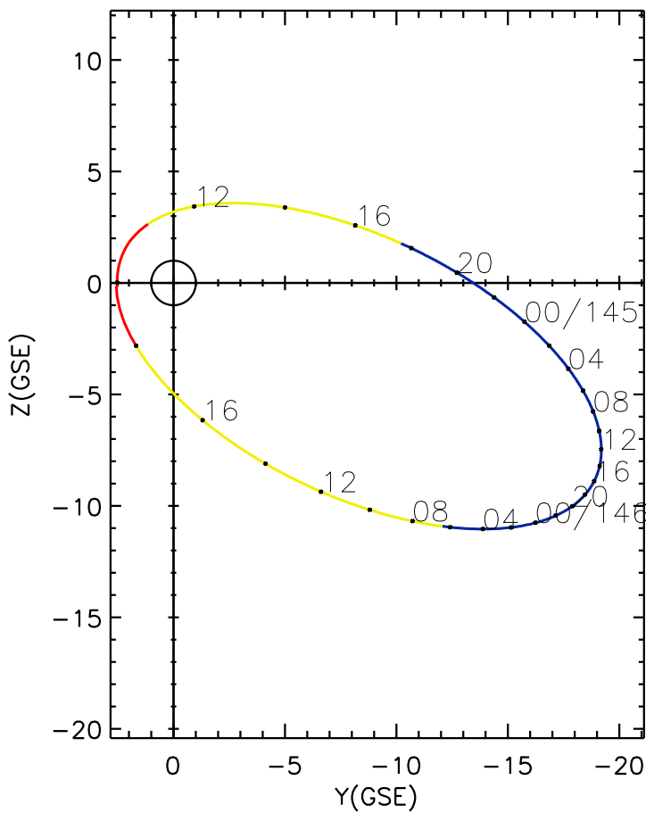
CLUSTER 2 orbit 2008 144 (05/23) 09:56 UT to 2008 146 (05/25) 19:01 UT
