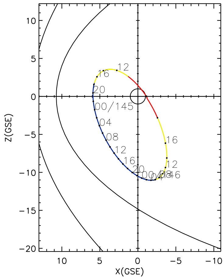
CLUSTER 2 orbit 2008 144 (05/23) 09:56 UT to 2008 146 (05/25) 19:01 UT
