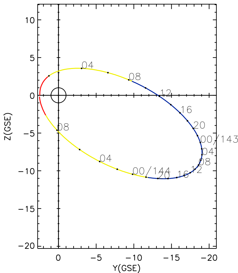
CLUSTER 2 orbit 2008 142 (05/21) 00:56 UT to 2008 144 (05/23) 09:56 UT
