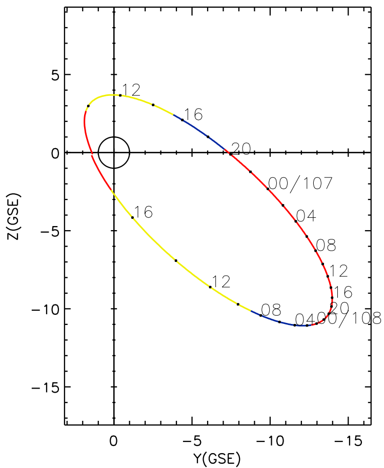
CLUSTER 2 orbit 2008 106 (04/15) 08:36 UT to 2008 108 (04/17) 17:41 UT
