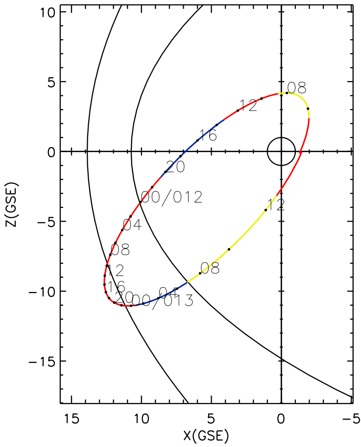
CLUSTER 2 orbit 2008 011 (01/11) 04:36 UT to 2008 013 (01/13) 13:46 UT
