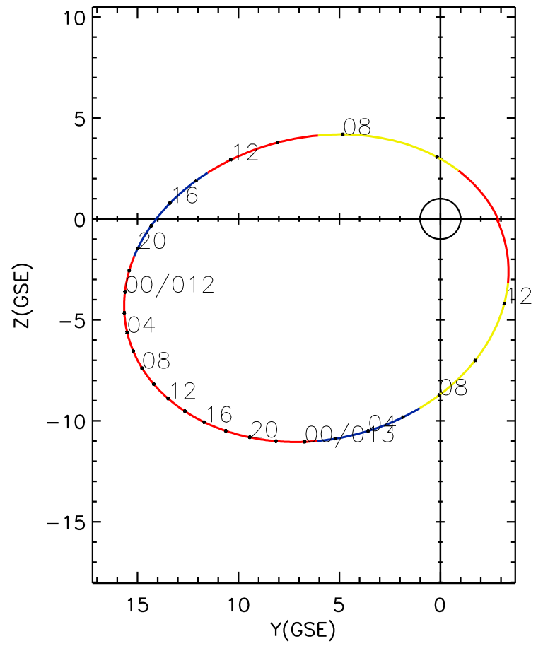
CLUSTER 2 orbit 2008 011 (01/11) 04:36 UT to 2008 013 (01/13) 13:46 UT
