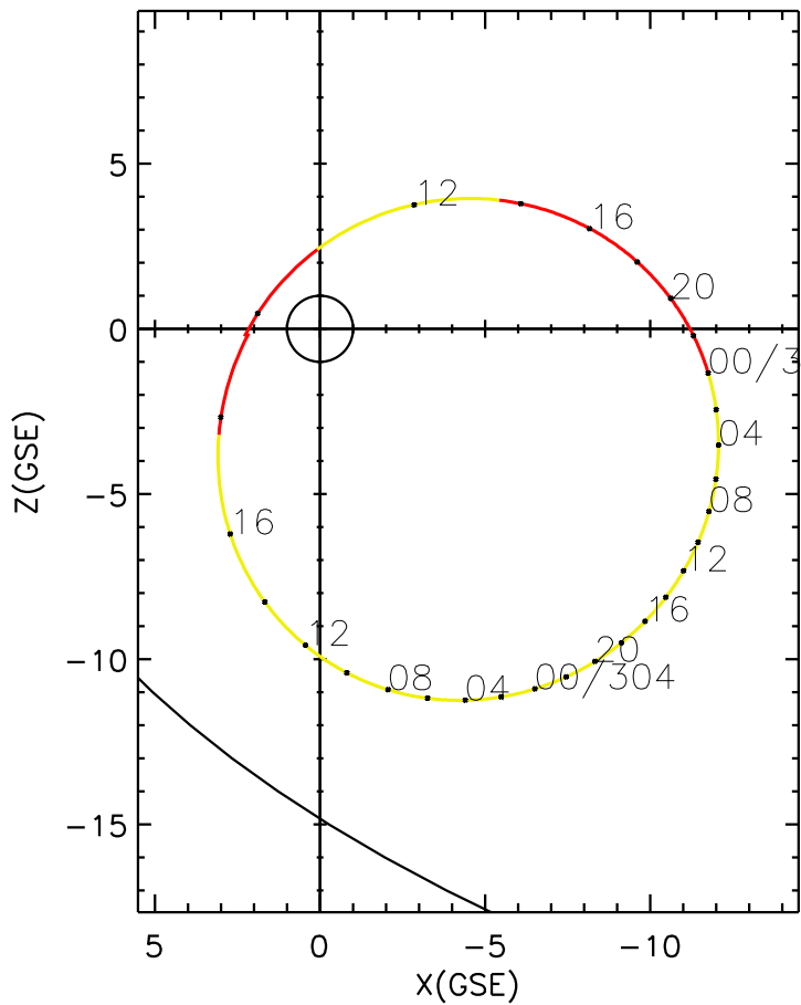
CLUSTER 2 orbit 2007 302 (10/29) 09:46 UT to 2007 304 (10/31) 18:56 UT
