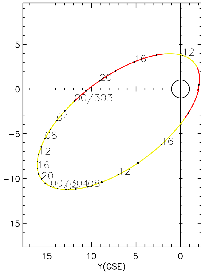
CLUSTER 2 orbit 2007 302 (10/29) 09:46 UT to 2007 304 (10/31) 18:56 UT
