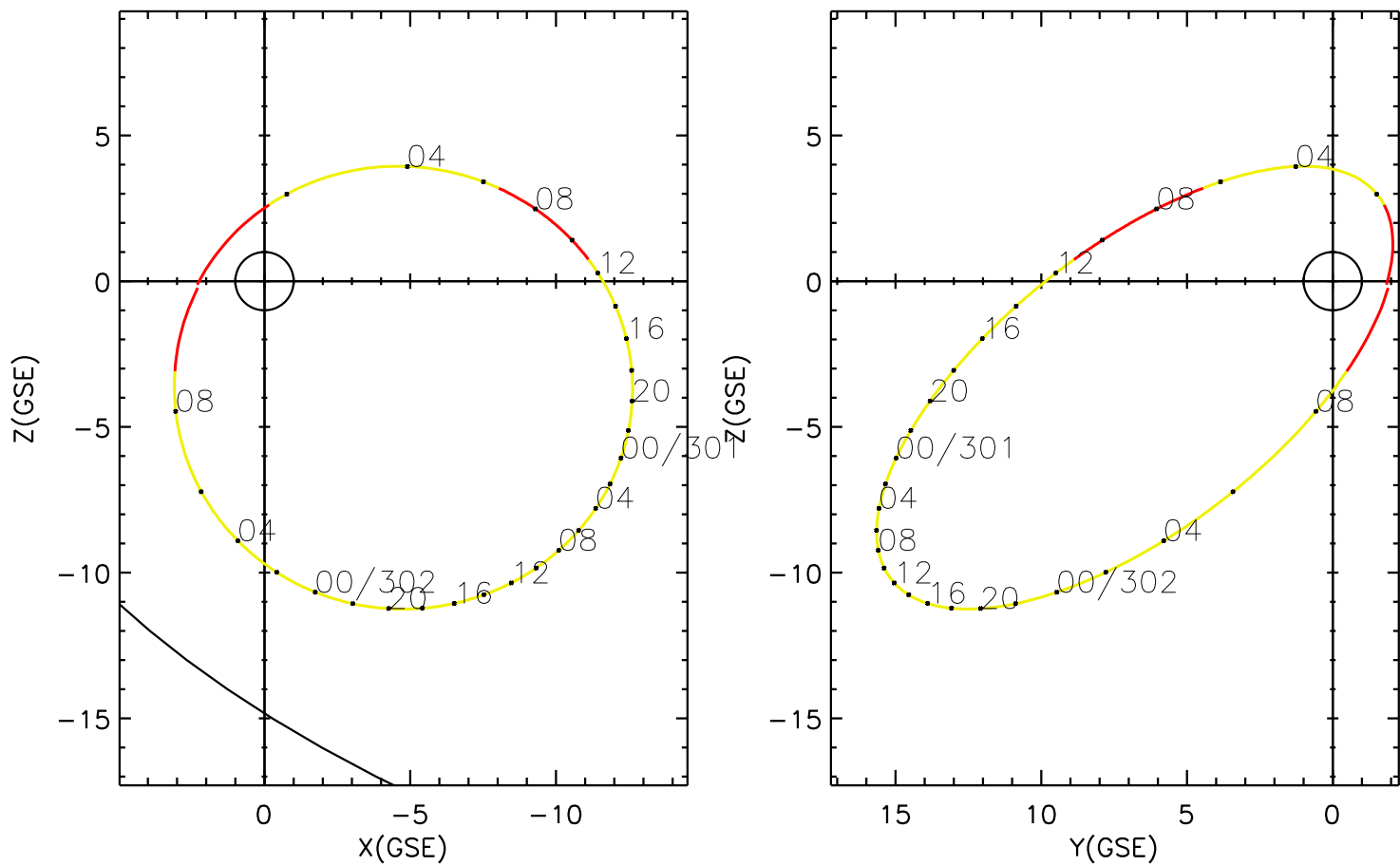
CLUSTER 2 orbit 2007 300 (10/27) 00:41 UT to 2007 302 (10/29) 09:46 UT
