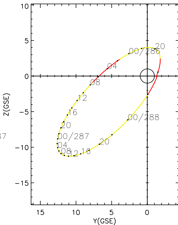
CLUSTER 2 orbit 2007 285 (10/12) 17:46 UT to 2007 288 (10/15) 02:56 UT
