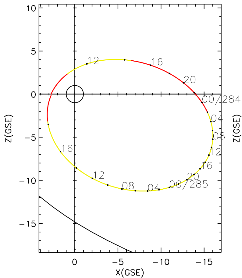
CLUSTER 2 orbit 2007 283 (10/10) 10:15 UT to 2007 285 (10/12) 19:20 UT
