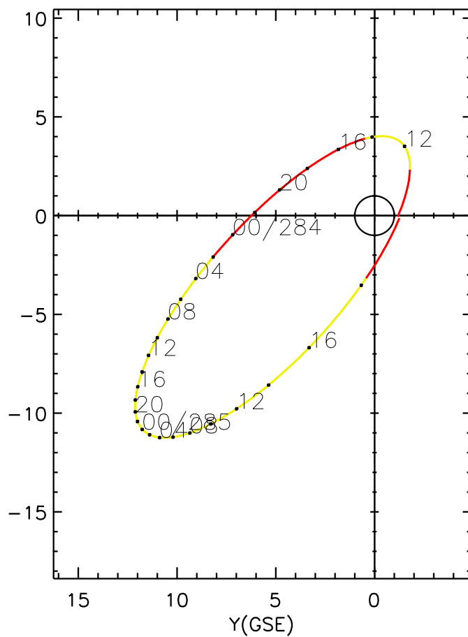
CLUSTER 2 orbit 2007 283 (10/10) 10:15 UT to 2007 285 (10/12) 19:20 UT
