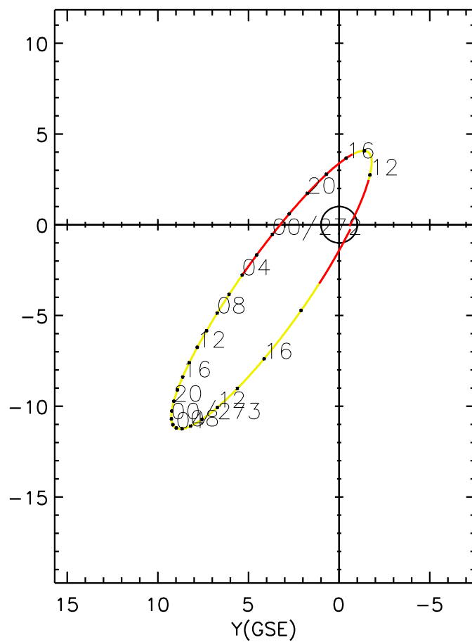
CLUSTER 2 orbit 2007 271 (09/28) 10:51 UT to 2007 273 (09/30) 19:56 UT
