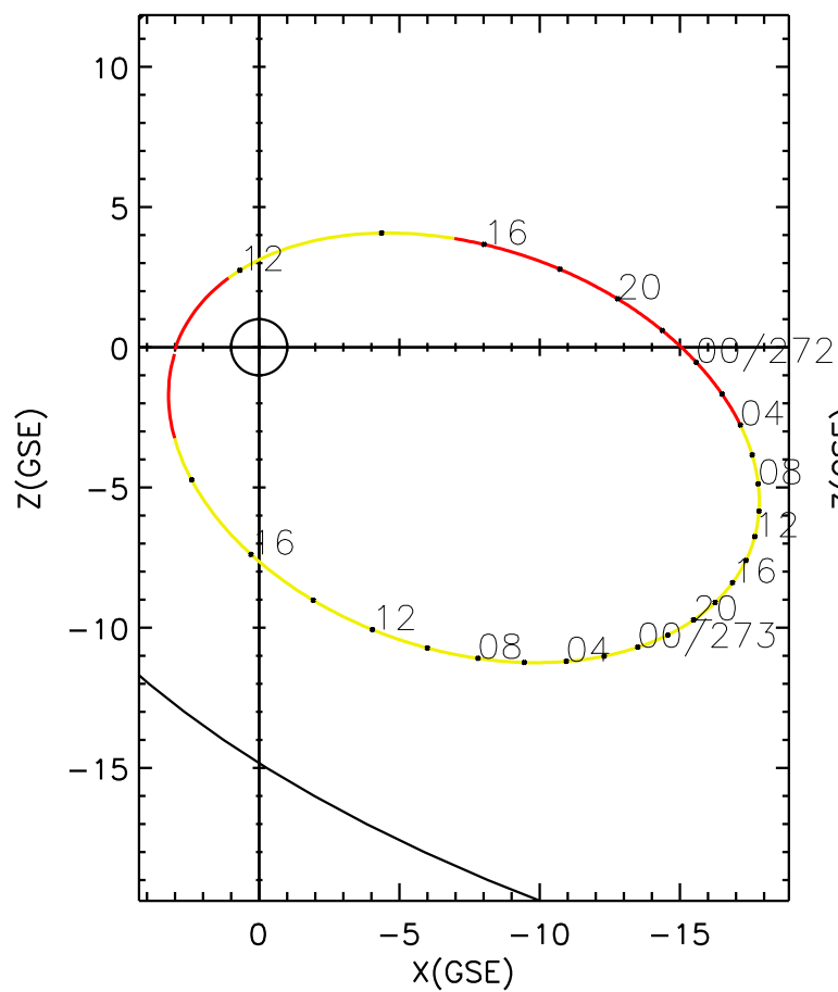
CLUSTER 2 orbit 2007 271 (09/28) 10:51 UT to 2007 273 (09/30) 19:56 UT
