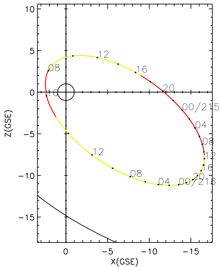
CLUSTER 2 orbit 2007 214 (08/02) 06:56 UT to 2007 216 (08/04) 16:06 UT
