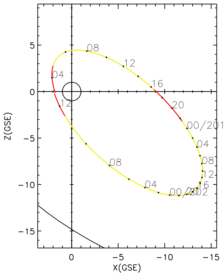
CLUSTER 2 orbit 2007 200 (07/19) 03:25 UT to 2007 202 (07/21) 12:30 UT
