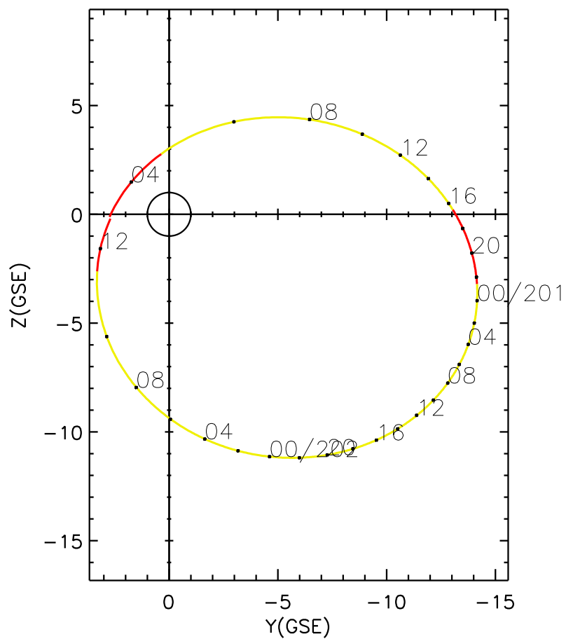
CLUSTER 2 orbit 2007 200 (07/19) 03:25 UT to 2007 202 (07/21) 12:30 UT
