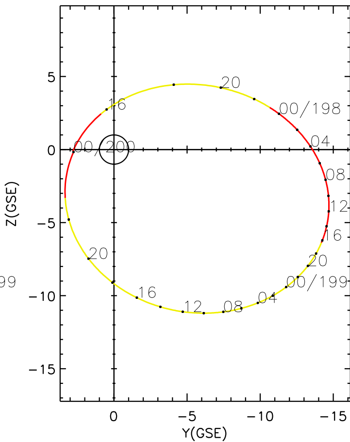
CLUSTER 2 orbit 2007 197 (07/16) 14:51 UT to 2007 200 (07/19) 00:01 UT
